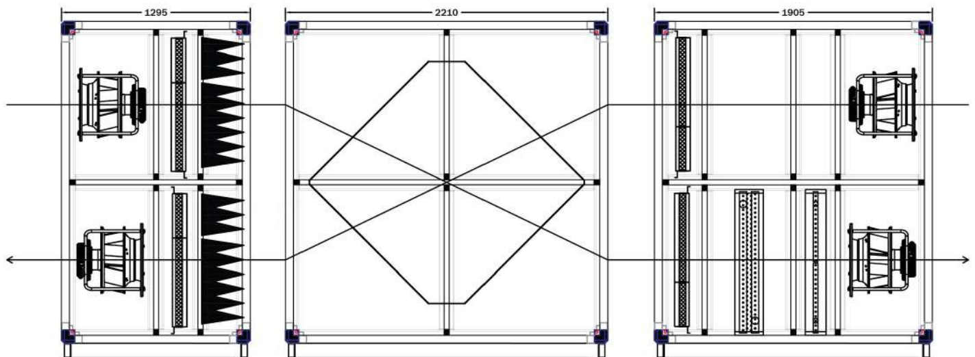
SIDE VIEW
